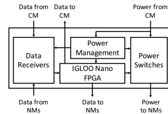
Fig. 3. Block diagram of Aggregator Module (AM).
